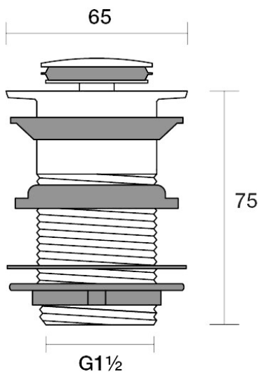
Universal Waste 40mm Pop - Up F11.023.1.43 - Brass
