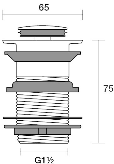
Universal Waste 40mm Pop - Up F11.023.1.57 - Matt Nickel
