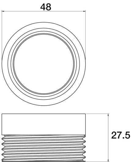
Universal Waste Adaptor 32mm to 40mm F11.041.1.40 - Rumbled Brass
