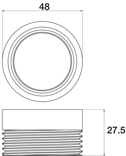
Universal Waste Adaptor 32mm to 40mm F11.041.1.45 - Native Brass
