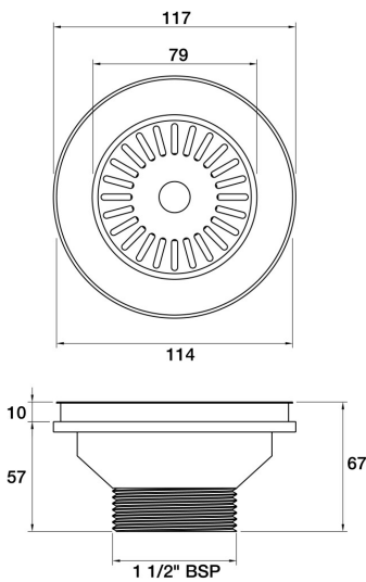
Universal Sink Basket F11.061.1.23 - Gunmetal
