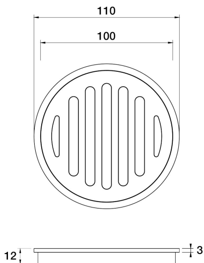
Universal Floor Grates Round 100mm Drop In Type F11.071.1.11 - 23k Gold
