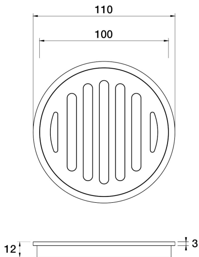
Universal Floor Grates Round 100mm Drop In Type F11.071.1.27 - Satin Pearl
