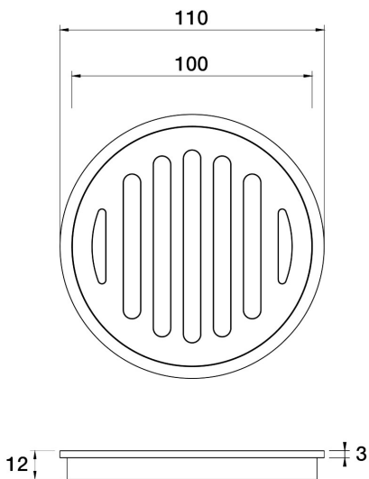
Universal Floor Grates Round 100mm Drop In Type F11.071.1.32 - Midnight Black
