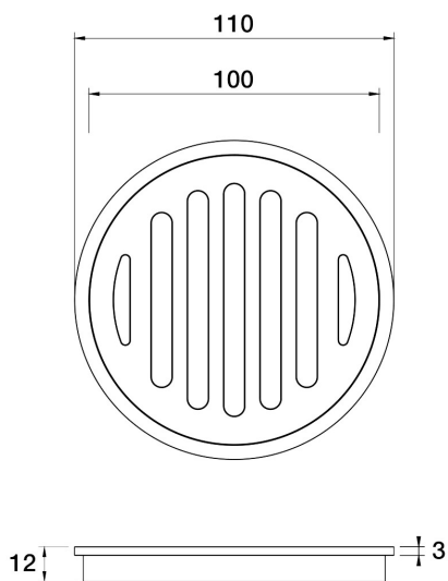
Universal Floor Grates Round 100mm Drop In Type F11.071.1.54 - Volcanic Grey
