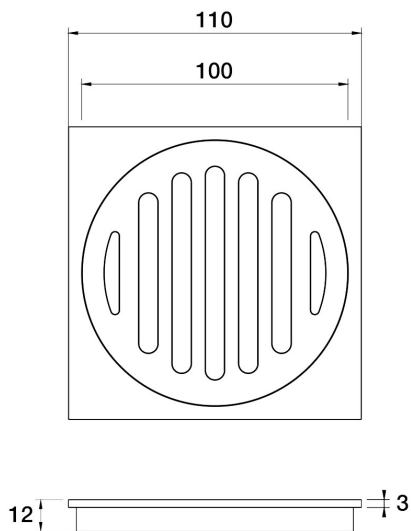
Universal Floor Grates Square 100mm F11.072.1.23 - Gunmetal
