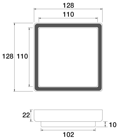
Universal Floor Grates Square 100mm Tile Insert F11.072.2.43 - Brass
