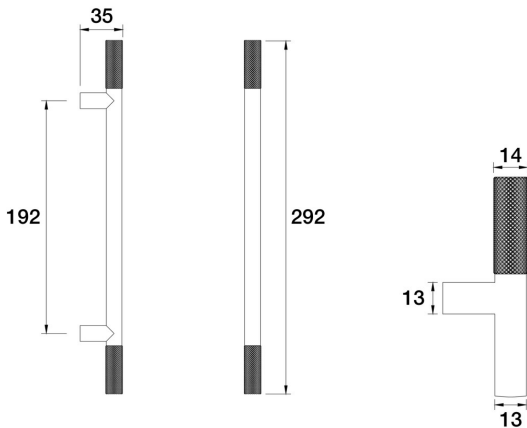
Elm Pull Handles Handle 192mm Centre H40.011.3.02 - Brushed Chrome
