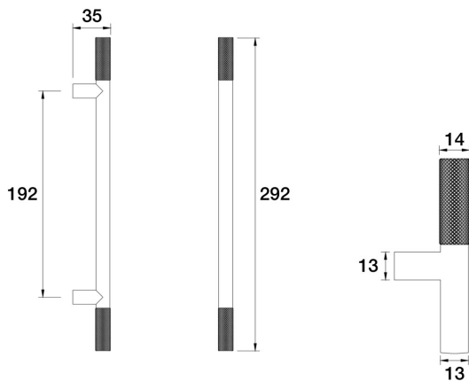
Elm Pull Handles Handle 192mm Centre H40.011.3.11 - 23k Gold
