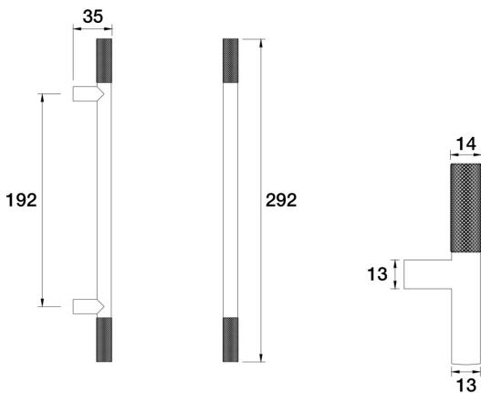
Elm Pull Handles Handle 192mm Centre H40.011.3.12 - 23k Brushed Gold
