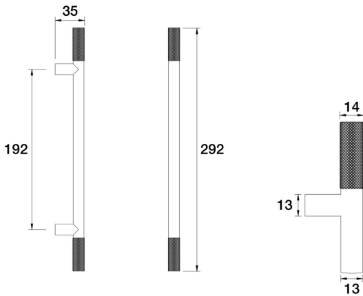
Elm Pull Handles Handle 192mm Centre H40.011.3.44 - Antique Copper
