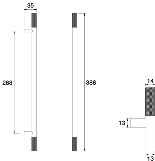
Elm Pull Handles Handle 288mm Centre H40.011.4.67 - Vintage Brass
