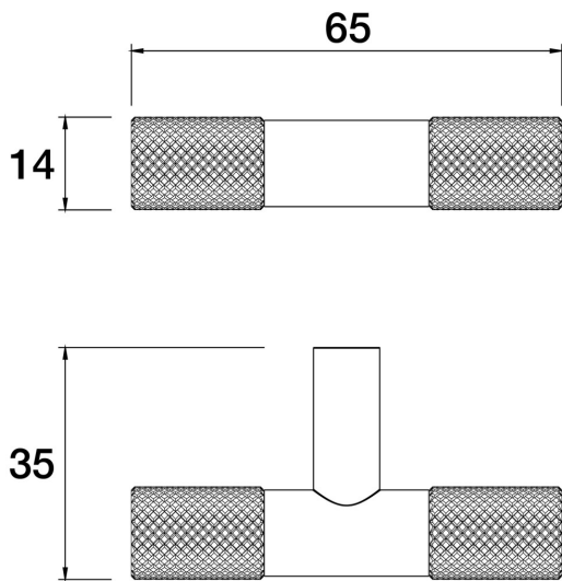
Elm Pull Handles Handle T Bar H40.011.5.24 - Brushed Gunmetal
