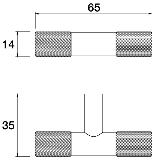
Elm Pull Handles Handle T Bar H40.011.5.40 - Rumbled Brass
