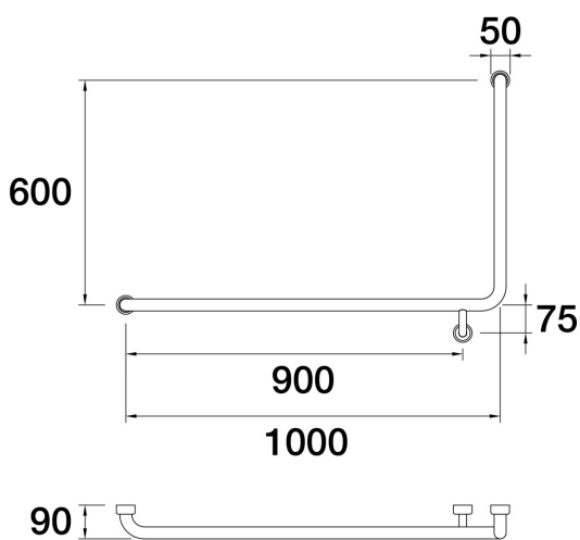
Universal Toilet Grab Rail 90° RH 1000mm x 600mm P10021.26 - Black Sapphire
