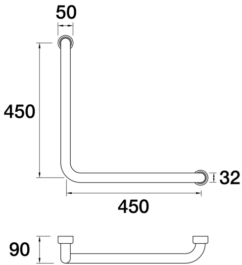
Universal Ambulant Grab Rail 450mm x 450mm I11.031.1.48 - Copper
