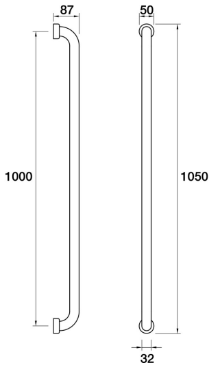
Universal Hand Shower Grab rail I11.041.1.32 - Midnight Black
