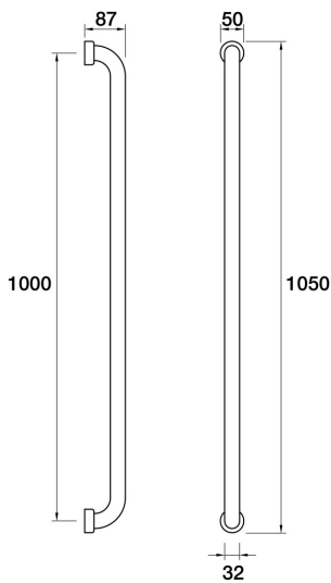
Universal Hand Shower Grab rail I11.041.1.48 - Copper
