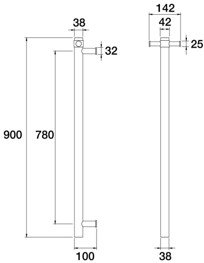
Lugano Heated Towel Rail Vertical 900mm
