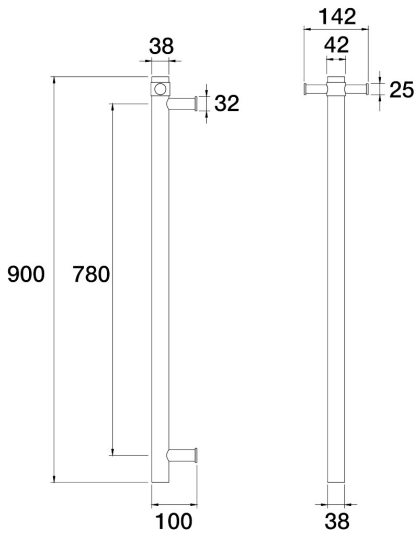
Lugano Heated Towel Rail Vertical 900mm J22.073.1.19 - 23k Brushed Brass Gold
