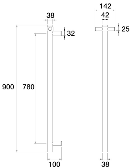
Lugano Heated Towel Rail Vertical 900mm J22.073.1.47 - Luminick
