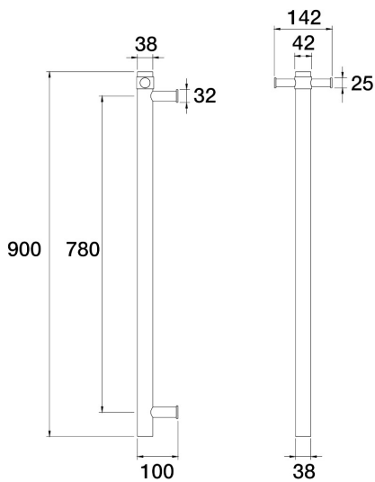
Lugano Heated Towel Rail Vertical 900mm J22.073.1.57 - Matt Nickel
