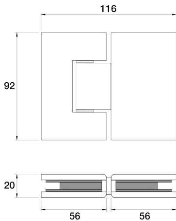
Universal Shower Hinge - 180° L11.011.1.11 - 23k Gold
