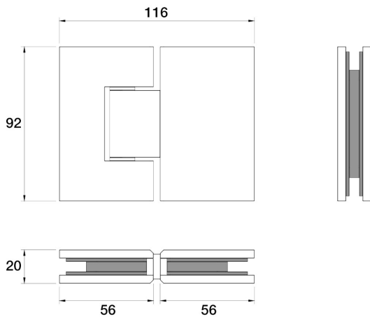
Universal Shower Hinge - 180° L11.011.1.24 - Brushed Gunmetal
