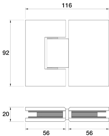
Universal Shower Hinge - 180° L11.011.1.34 - Matt Black
