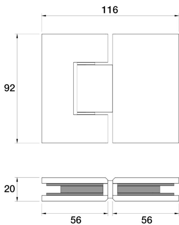
Universal Shower Hinge - 180° L11.011.1.43 - Brass
