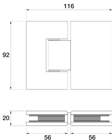
Universal Shower Hinge - 180° L11.011.1.48 - Copper
