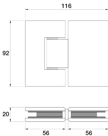
Universal Shower Hinge - 180° L11.011.1.54 - Volcanic Grey
