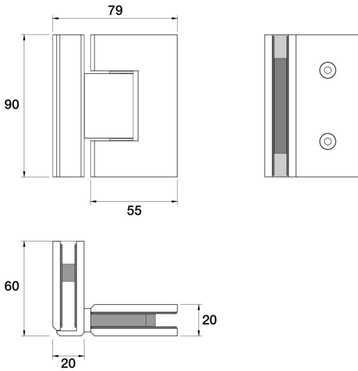
Universal Shower Hinge - 90° L11.011.2.01 - Chrome
