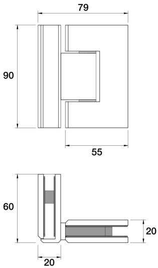
Universal Shower Hinge - 90° L11.011.2.01 - Chrome
