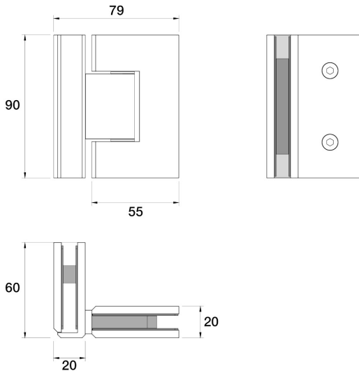
Universal Shower Hinge - 90° L11.011.2.19 - 23k Brushed Brass Gold
