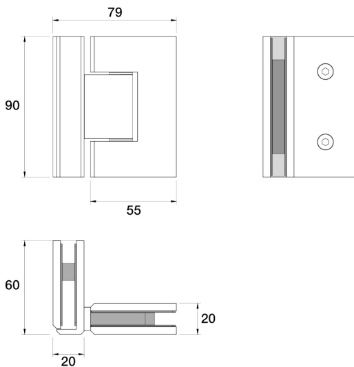
Universal Shower Hinge - 90° L11.011.2.32 - Midnight Black
