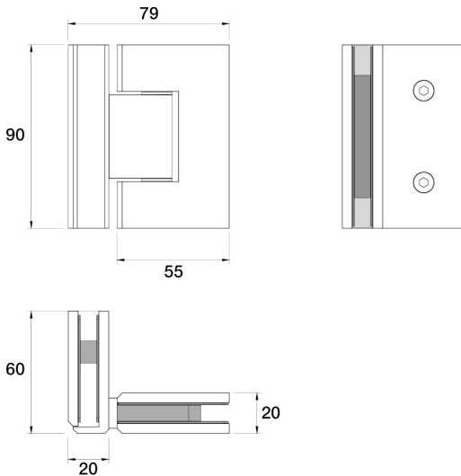
Universal Shower Hinge - 90° L11.011.2.45 - Native Brass
