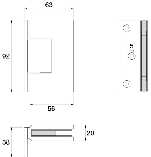
Universal Shower Hinge - Wall to Glass 90° L11.011.3.32 - Midnight Black
