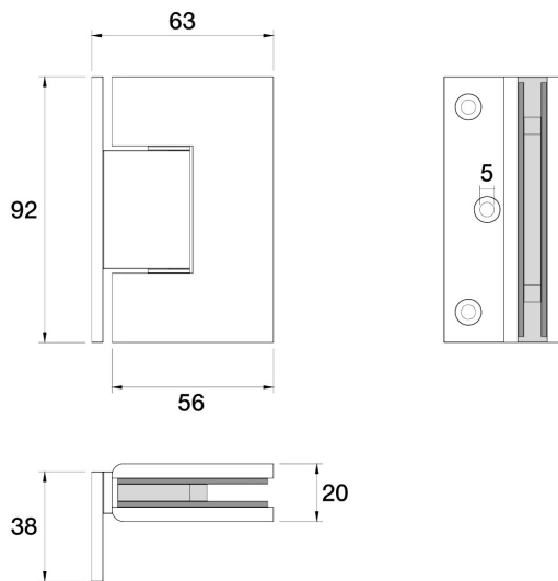
Universal Shower Hinge - Wall to Glass 90° L11.011.3.40 - Rumbled Brass
