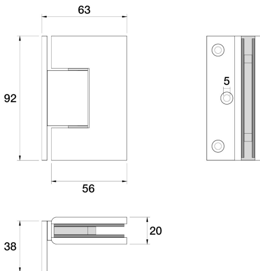
Universal Shower Hinge - Wall to Glass 90° L11.011.3.48 - Copper
