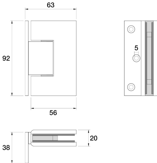
Universal Shower Hinge - Wall to Glass 90° L11.011.3.57 - Matt Nickel
