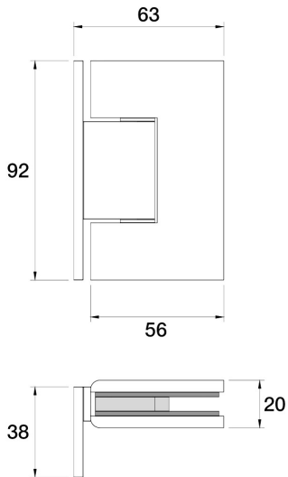
Universal Shower Hinge - Wall to Glass 90° L11.011.3.68 - Autumn Bronze
