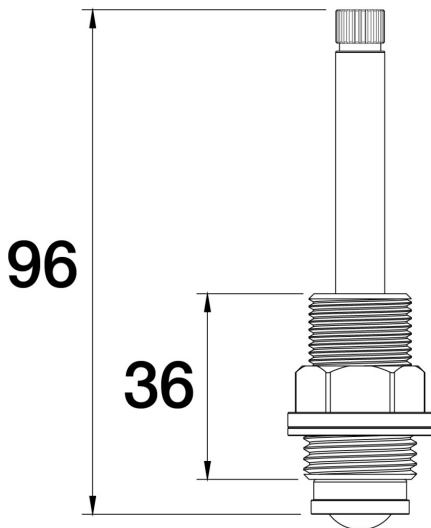
Portsea / Forme / Poem Hob 86mm x 36mm Spindles - Spline P01.006.32 - Midnight Black
