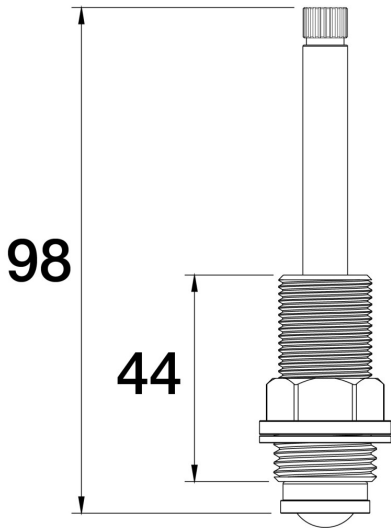
Portsea / Forme / Poem Wall 98mm x 44mm Spindles - Spline P01.007.01 - Chrome
