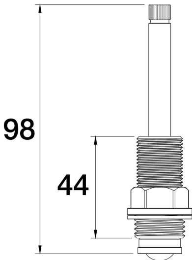
Portsea / Forme / Poem Wall 98mm x 44mm Spindles - Spline P01.007.23 - Gunmetal
