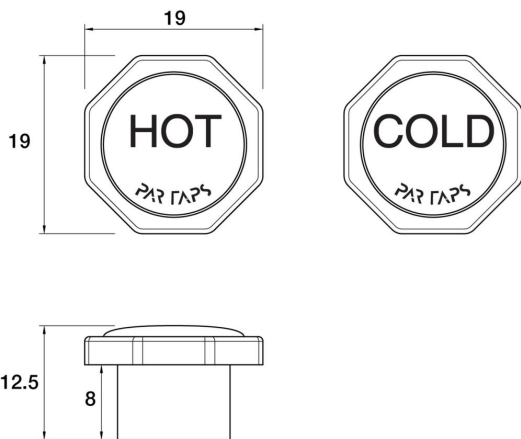
Hot & Cold Buttons - Chrome P01.012.32 - Midnight Black
