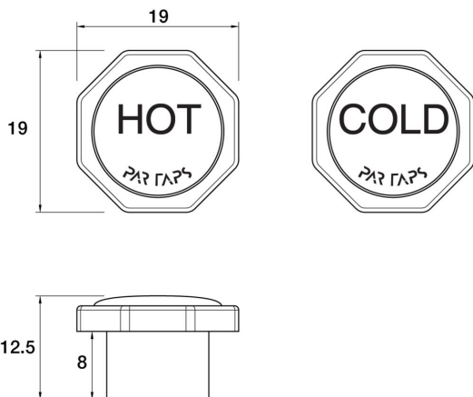
Hot & Cold Buttons - Chrome P01.012.34 - Matt Black
